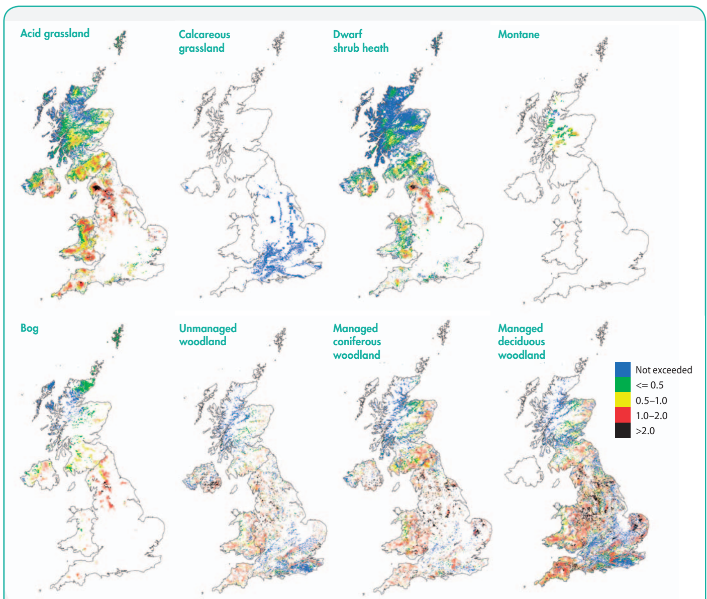
Figure 14.5 Exceedance of the critical loads of acidity for UK broad habitats by acid deposition for 2006–2008. The critical loads of acidity are determined by the buffering capacity of the dominant soil type in each 1x1 km square and habitat-specific parameters. Source: Centre for Ecology and Hydrology; Hall et al. (2003, 2004, 2008, 2009); http://cldm.defra.gov.uk
